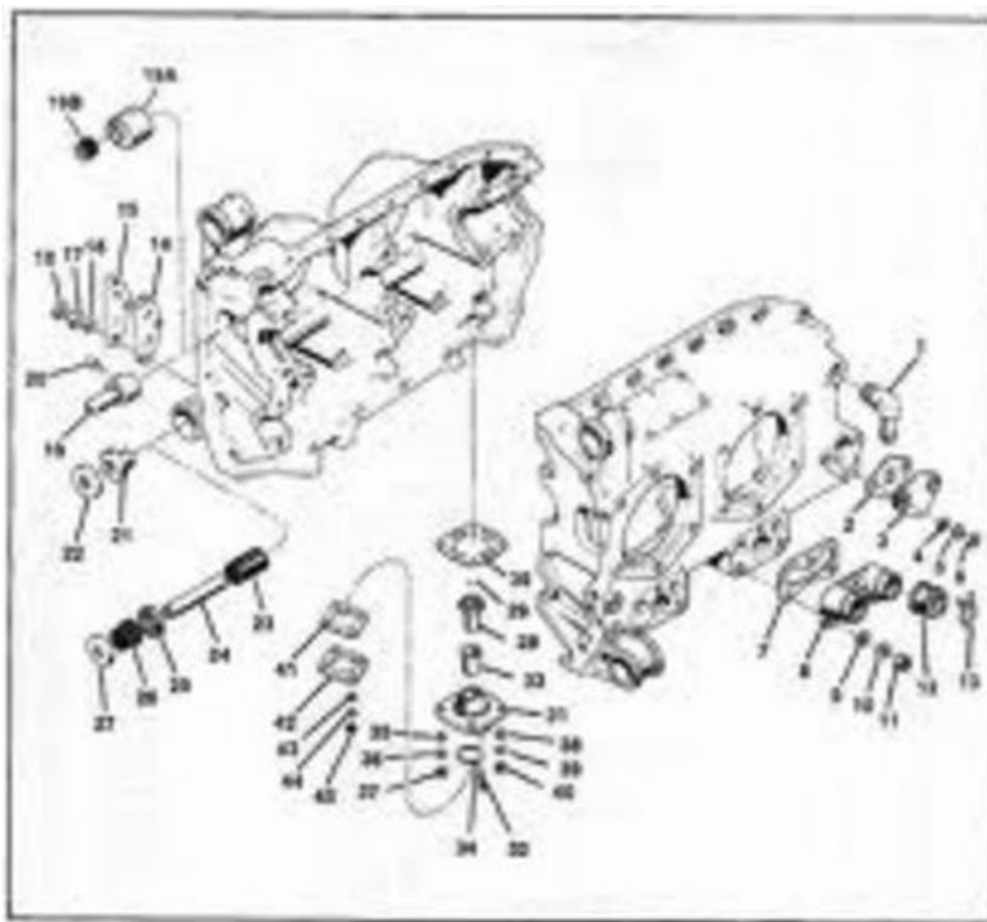
FIGURE 3. CRANKCASE ASSOCIATED PARTS
